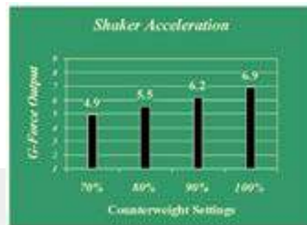
5000 BLE-18X Series Actual G-Force Reading
